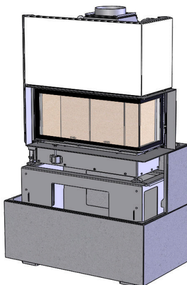
Illustration 13: Put the Architecture corner fireplace on top of the support bearing
