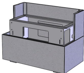
Illustration 12: Set up the back wall element
