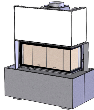
Illustration 5: Place the lower segments onto the bottom plate
