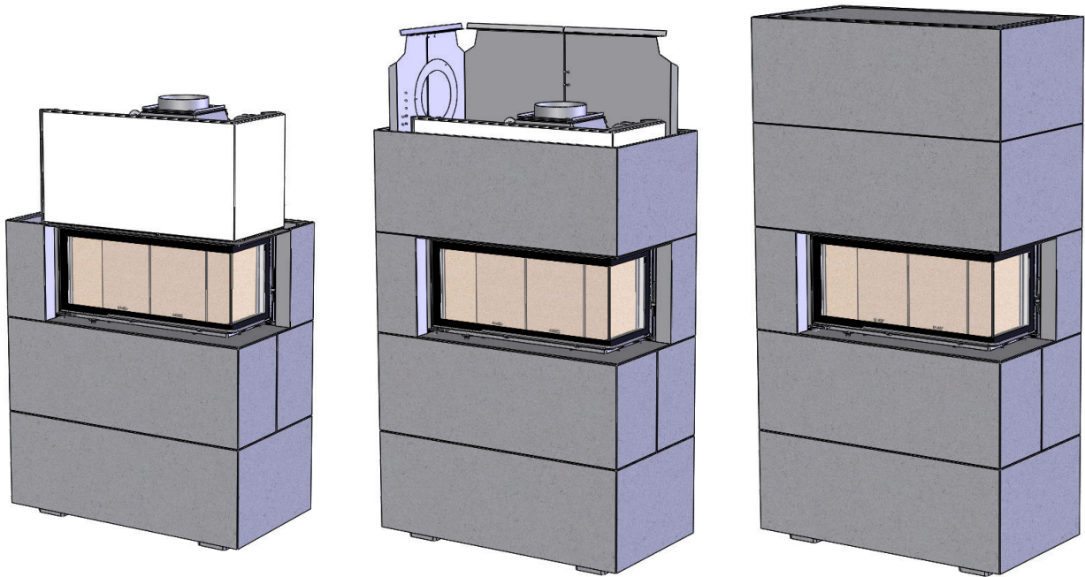
Illustration 15: Lift the fireplace enclosure over the fireplace and apply it on the lower elements
