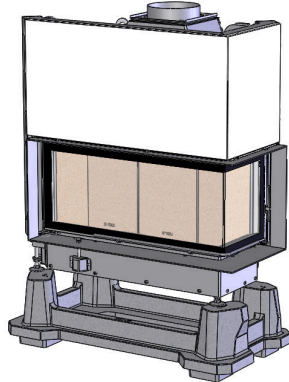
Illustration 4: Place the Corner fire-plate onto the bottom plate and align it
